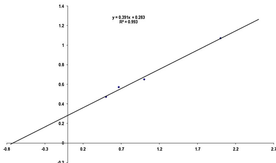
Fig. 4. Lineweaver-Burk plot of purified \alpha -amylase from A. flavithermus .
